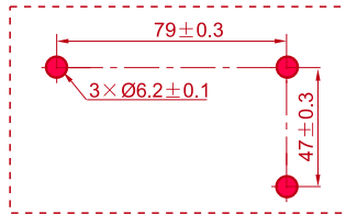
Mounting hole size
